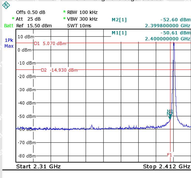
GFSK Transmitting Band edge-left side
